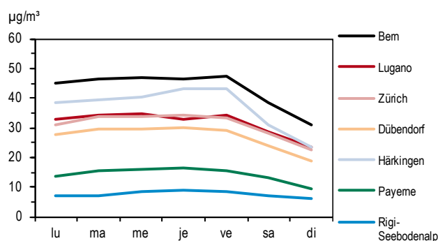
Figure 11 > Dioxyde d'azote (NO 2 ), fluctuations hebdomadaires, 2013
