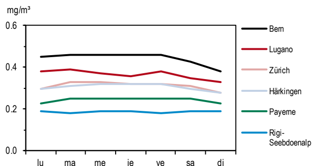
Figure 38 > Fluctuations hebdomadaires (CO), 2013
