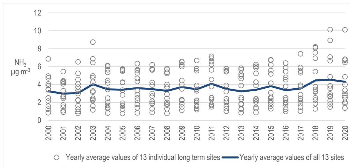
Fig. S 1 Annual mean of ammonia concentrations Average (solid line) and single values (circles) of the annual mean ammonia concentrations from all 13 sites with continuous measurements since 2000.
