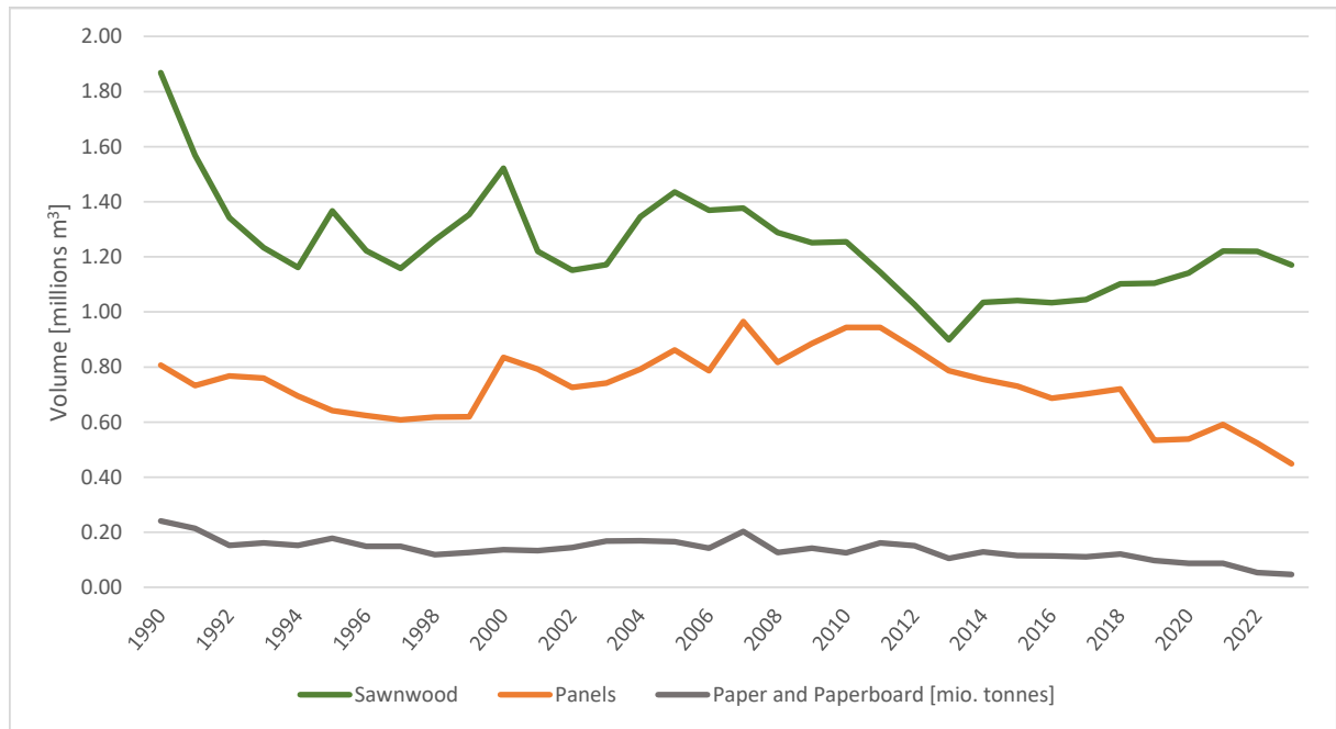
Figure 4: Production of HWP from domestic harvesting (sawnwood and panels in millions of m³, paper and paperboard in millions of tonnes); 1990-2022. The share of recovered fibre pulp in paper production is excluded.
