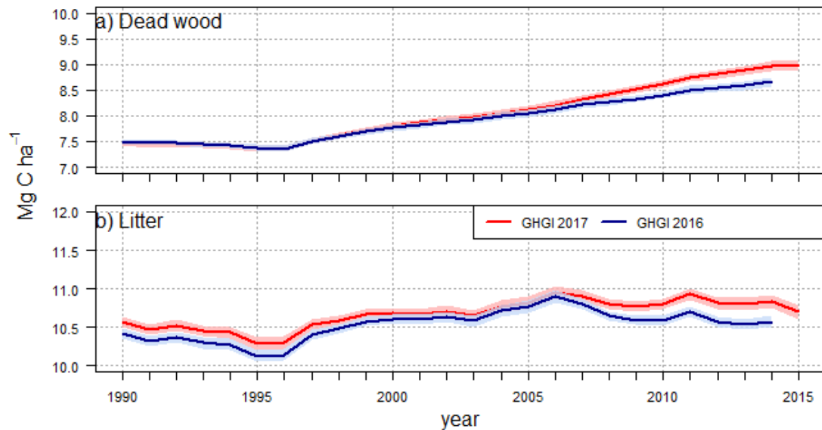
Figure 7. Mean (solid line) and double standard error (shaded area) of carbon stocks for the litter and dead wood pools in the GHGI 2016 and 2017.
