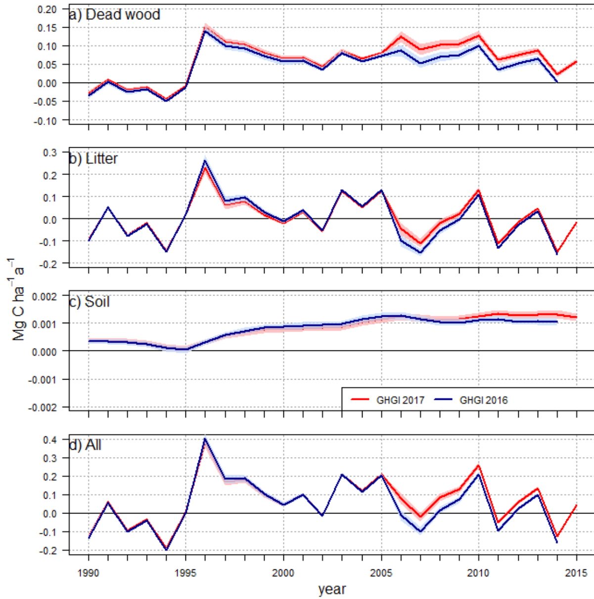
Figure 6. Mean (solid line) and double standard error (shaded area) of carbon stock change for three pools soil, litter, dead wood and their sum (ALL) in the GHGI 2016 and 2017. Negative values indicate C losses, positive values C gains.
