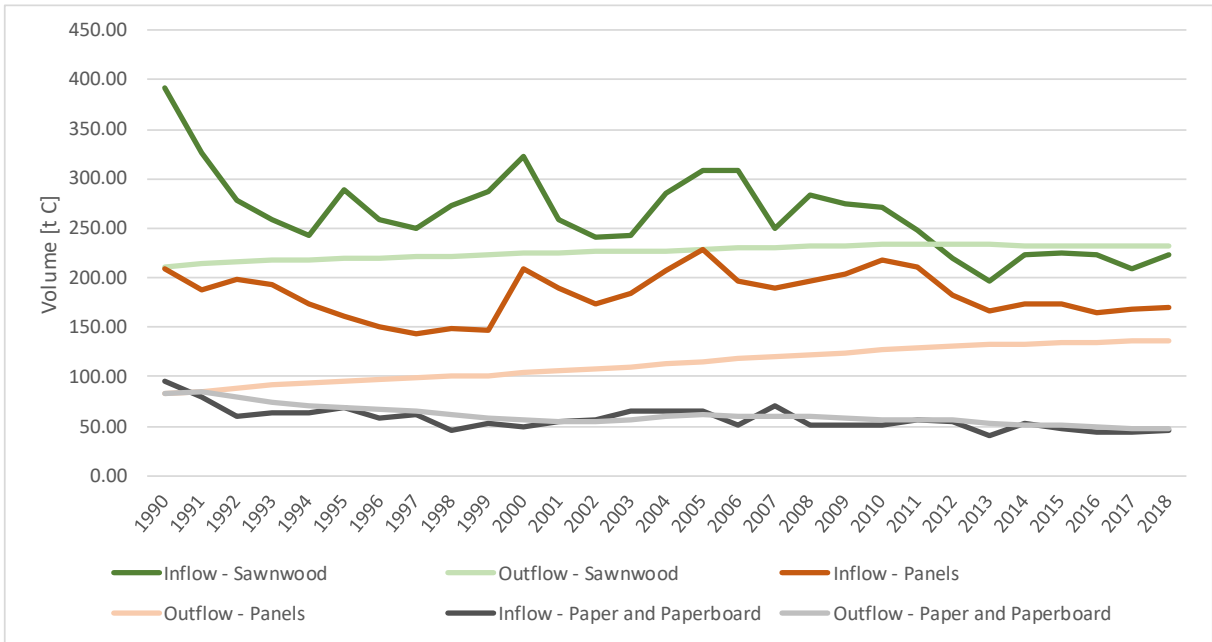
Figure 4: Inflow and outflow from the HWP pool for the categories sawnwood and panels; 1990-2018.
