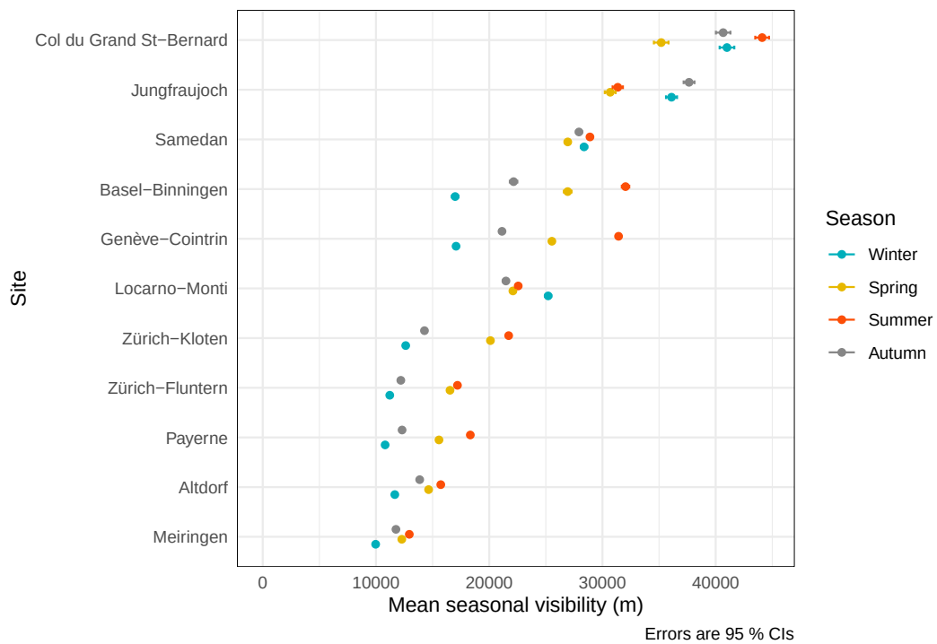
Figure 6: Mean seasonal visibility between 1980 and 2018 for 11 visibility monitoring sites in Switzerland. Sites are ordered by their overall mean visibility.
