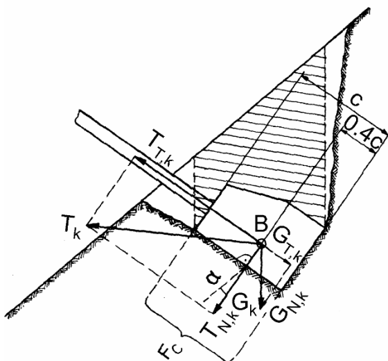
Fig. 35 > Dimensioning of upper concrete foundations to withstand compression forces.
