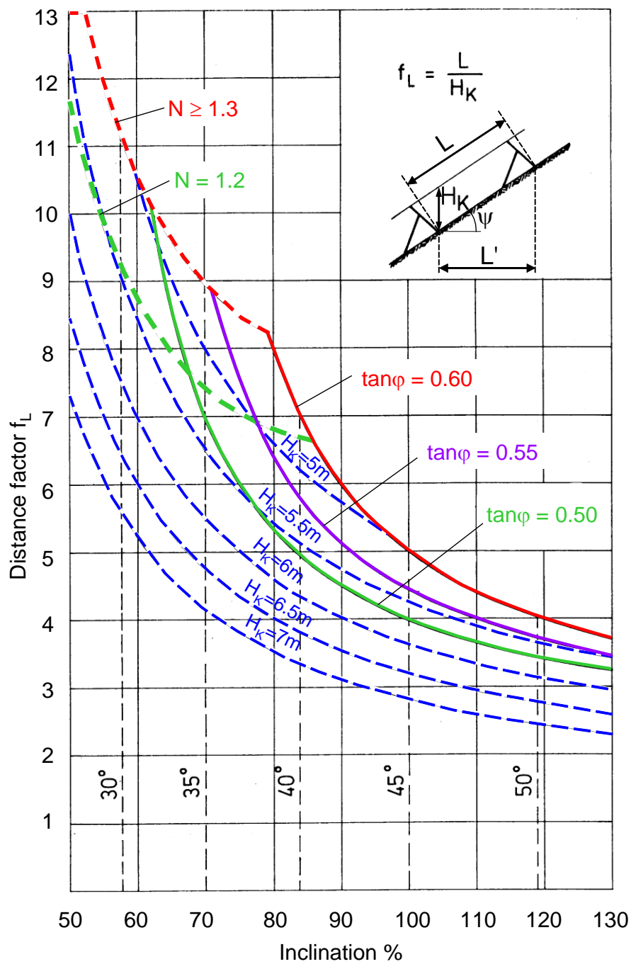
Fig. 13 > Distance factor f_L .
