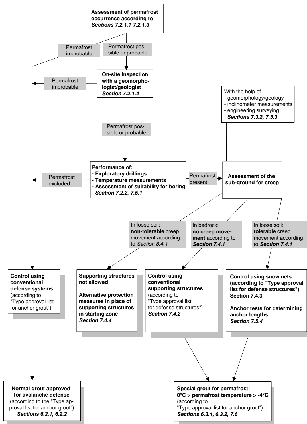
Fig. 53 > Flow diagram.
