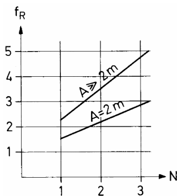
Fig. 19 > End-effect factor as specified by equation (22).
