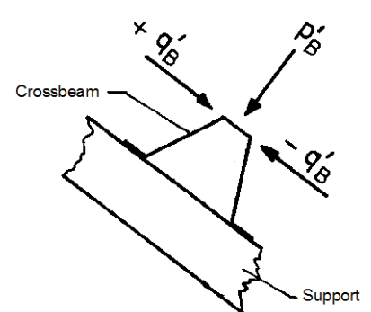
Fig. 26 > Loading widths for crossbeams. Fig. 27 > Forces parallel to the plane of the grate. Fig. 28 > Transverse load on crossbeam.
