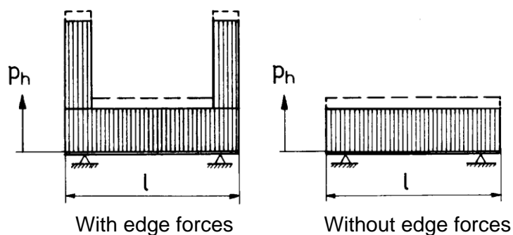
Fig. 25 > Load cases with and without end-effect loads.
