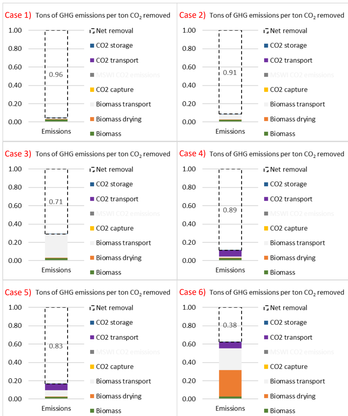
Figure 7.5: LCA results (climate impacts: tons of GHG emissions per ton of CO 2 permanently removed from the atmosphere) for different BECCS configurations (wood combustion with CCS), as generated with the LCA tool and specified in Table 7.6. Numbers in the dashed bar segments on top of the emissions indicate net CO 2 removal rates. Wood power plant operation in Switzerland in all cases; CO 2 storage in Switzerland (cases 1-3) and Iceland (cases 4-6).
