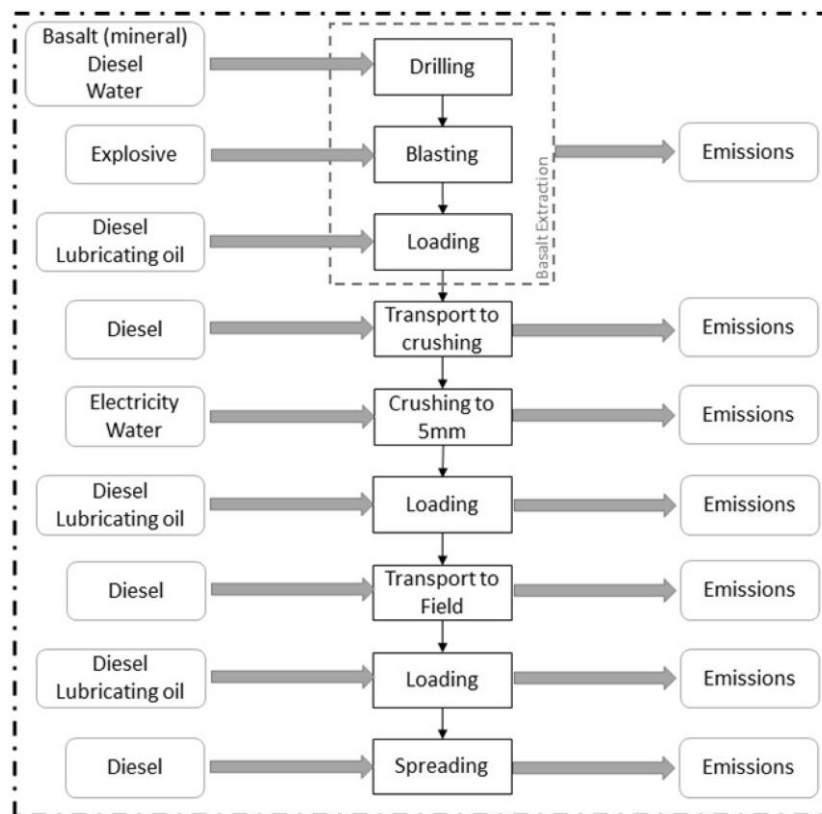
Figure 6.10: System boundaries of a typical enhanced weathering system including extraction, comminution, transport and spreading of basalt (Lefebvre et al. , 2019).
