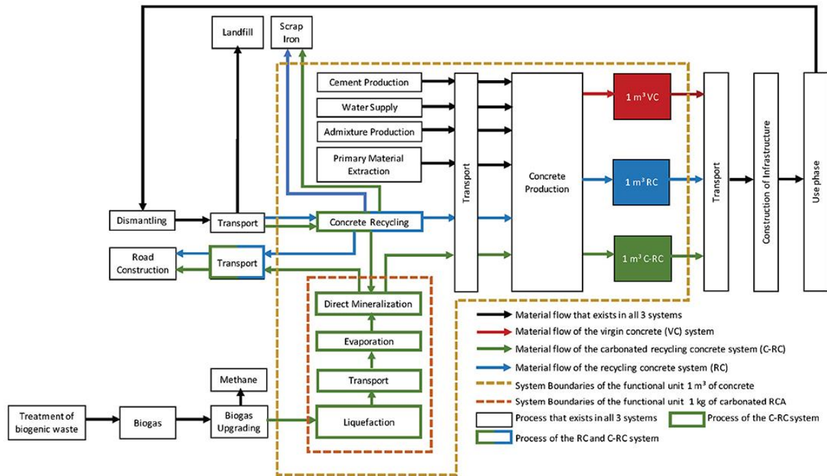
Figure 6.8: System boundaries of the product system considered in our LCA (Tiefenthaler et al. , 2021), comparing production of virgin concrete (VC) without recycled fractions, recycled concrete (RC), and carbonated recycled concrete (C-RC). RCA: Recycled Concrete Aggregate.
