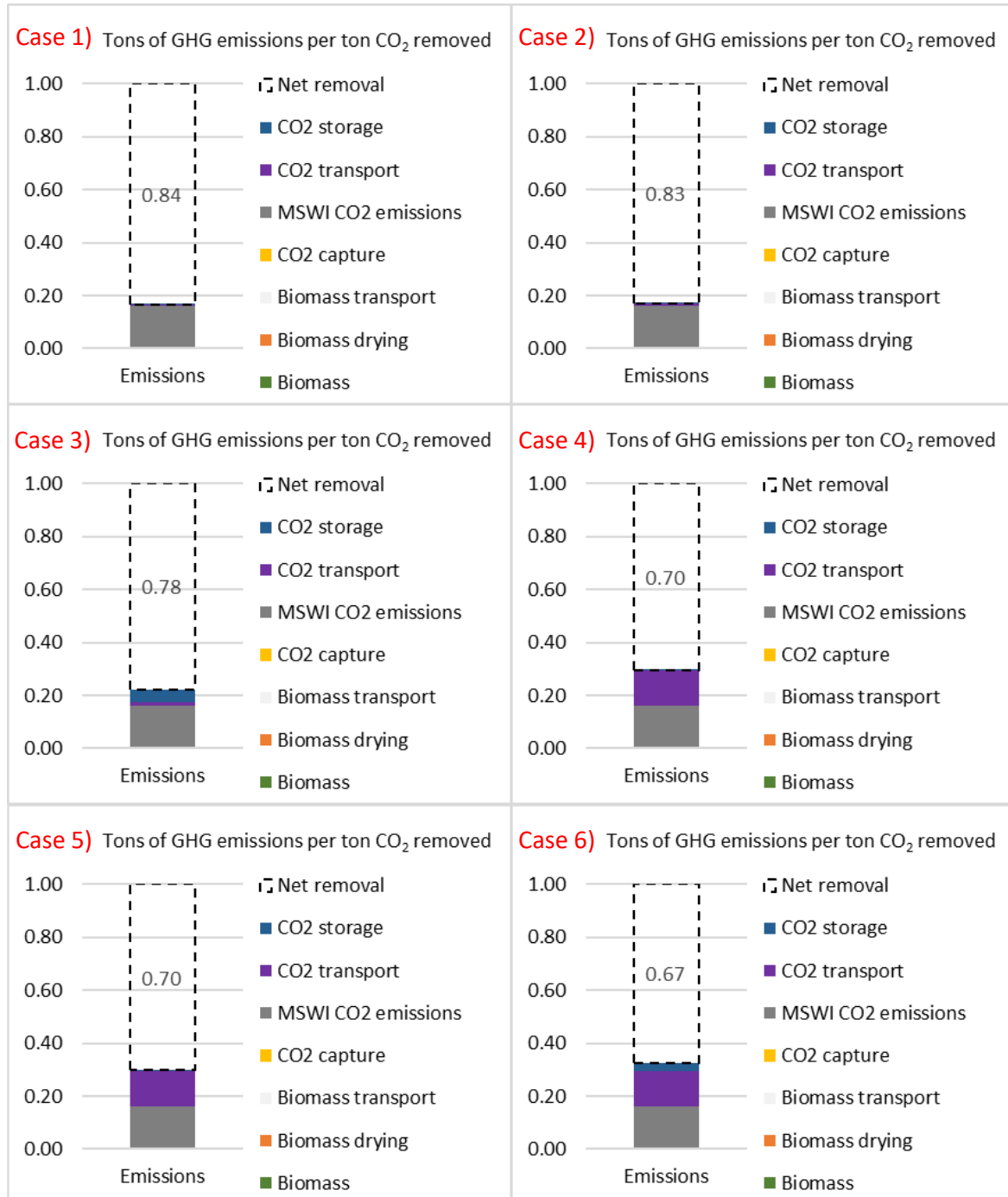
Figure 7.6: LCA results (climate impacts: tons of GHG emissions per ton of CO 2 permanently removed from the atmosphere) for different MSWI with CCS configurations, as generated with the LCA tool and specified in Table 7.8. Numbers in the dashed bar segments on top of the emissions indicate net CO 2 removal rates. MSWI operation in Switzerland in all cases; CO 2 storage in Switzerland (cases 1-3) and Iceland (cases 4-6). “Biomass” refers to the biogenic waste fraction. Only the fossil fraction of CO 2 emissions not captured at the MSWI plant generates climate impacts. Residual fossil CO 2 (not captured by the CO 2 capture unit) and downstream emissions are entirely assigned to CO 2 removal.
