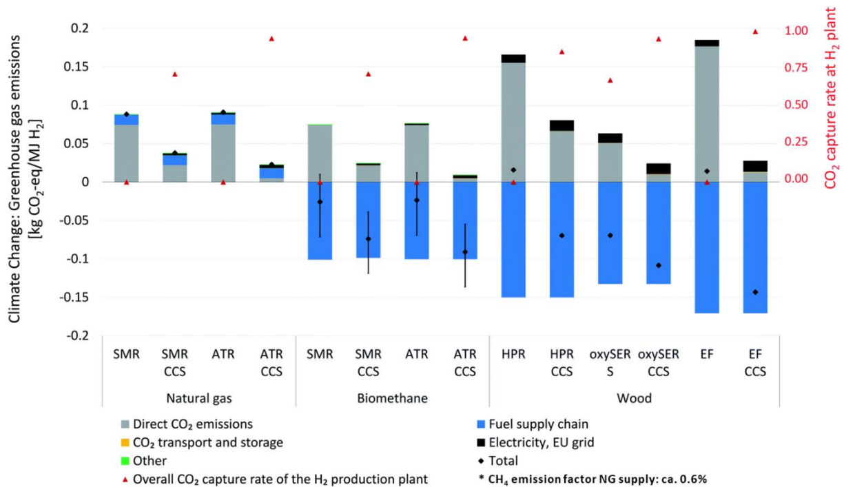
Figure 6.7: Impacts on climate change in terms of life-cycle GHG emissions due to hydrogen production from natural gas, biomethane and wood with and without CCS (Antonini et al., 2021). Error bars for the biomethane pathway indicate variability due to different disposal options for the digestate from the biogas production. SMR: Steam Methane Reforming; ATR: Autothermal Reforming; HPR: Heat Pipe Reformer; oxySER: Sorption enhanced reforming gasifier, EF: Entrained flow gasifier; EU grid: current average European electricity.
