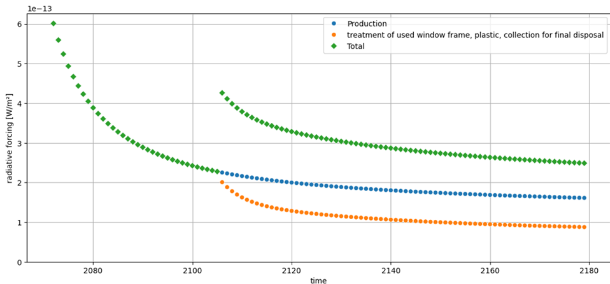
Figure 6.14: The radiative forcing profiles for the time explicit life cycle of a plastic window frame placed in 2075.
