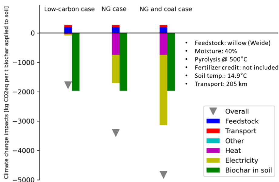
Figure 6.4: Impacts on climate change per ton of biochar applied to soil (Hoeskuldsdottir, 2022). NG: Natural gas. Specific cases here are primarily selected and shown to highlight the importance of substitution effects. “Biochar in soil” represents the amount of CO 2 permanently removed from the atmosphere, while the negative emissions from “heat” and “electricity” represent avoided emissions due to substitution of replaced energy supply.
