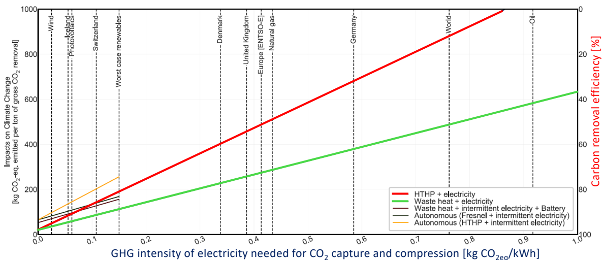
Figure 6.2: Life-cycle GHG emissions of a DACCS system as a function of the GHG emission intensity of the energy needed for operation of the DAC unit (Terlouw, Treyer, et al. , 2021). HTHP: High-temperature heat pump; “Fresnel”: Solar heat collector. Vertical dashed lines represent the average life cycle GHG emission intensities of technology- or country-specific electricity supply. Carbon removal efficiency refers to the net-effectiveness of permanent CO 2 removal considering all GHG emissions caused by the DACCS product system.
