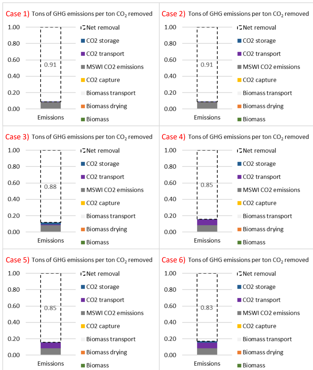
Figure 7.7: LCA results (climate impacts: tons of GHG emissions per ton of CO 2 permanently removed from the atmosphere) for different MSWI with CCS configurations, as generated with the LCA tool and specified in Table 7.8. Numbers in the dashed bar segments on top of the emissions indicate net CO 2 removal rates. MSWI operation in Switzerland in all cases; CO 2 storage in Switzerland (cases 1-3) and Iceland (cases 4-6). “Biomass” refers to the biogenic waste fraction. Only the fossil fraction of CO 2 emissions not captured at the MSWI plant generates climate impacts. Residual fossil CO 2 (not captured by the CO 2 capture unit) and downstream emissions are assigned to CO 2 removal according to the biogenic carbon fraction of the waste (52%).
