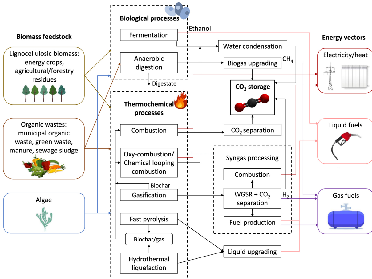
Figure 5.9: BECCS configurations and categorizations according to (Cobo et al., 2023). Note that “biochar” can be considered as BECCS option, but also as a CDR method on its own, mostly depending on whether biochar production and application is the main purpose of the process chain, or energy vector production with biochar as a by-product. 23
