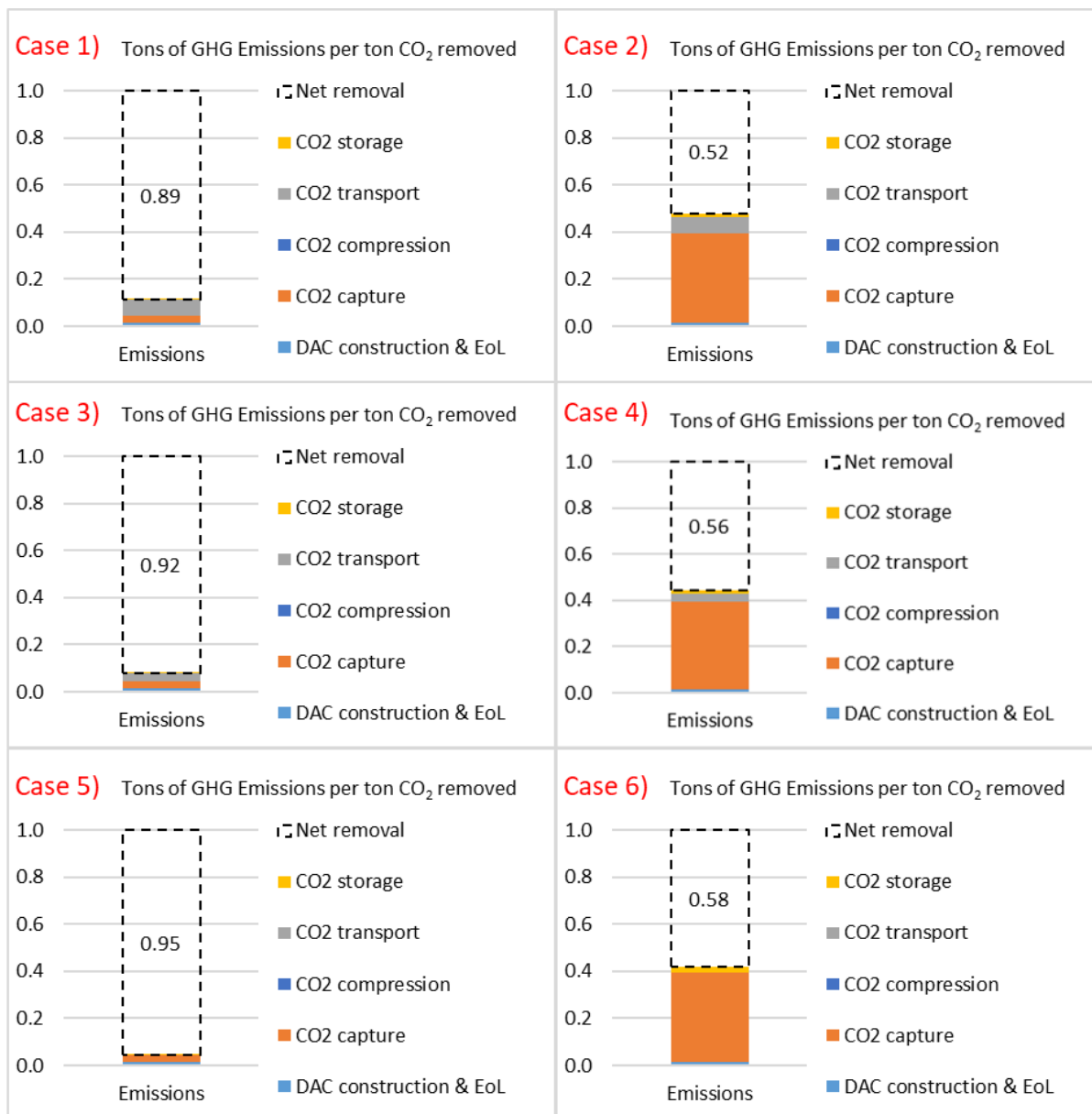
Figure 7.1: LCA results (climate impacts: tons of GHG emissions per ton of CO 2 permanently removed from the atmosphere) for different LT DACCS configurations with DAC operation in Switzerland, as generated with the LCA tool and specified above in Table 7.1. Location of CO 2 storage: Cases 1, 2: Iceland; cases 3, 4: Norway; cases 5, 6: Switzerland. Numbers in the dashed bar segments on top of the emissions indicate net CO 2 removal rates. Cases 2, 4, and 6 use natural gas as energy source for DAC operation.
