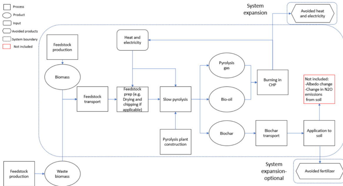
Figure 6.3: System boundaries of the biochar-to-soil LCA (Hoeskuldsdottir, 2022). The scheme does not include all potential side-effects such as impacts on soil biology, organic soil carbon, or contaminants.
