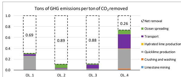
Figure 7.10: Comparison of life cycle GHG emissions and net CO 2 removal rates of different CDR methods with four specific parameter settings each, as specified in Table 7.12. Stacked colored bars show life cycle GHG emissions; numbers in the dashed bar segments on top of the emissions indicate net CO 2 removal rates. "By-products" of CDR, e.g., heat and electricity generation in case of BECCS and biochar application, are not shown here, but provided in Table 7.13.
