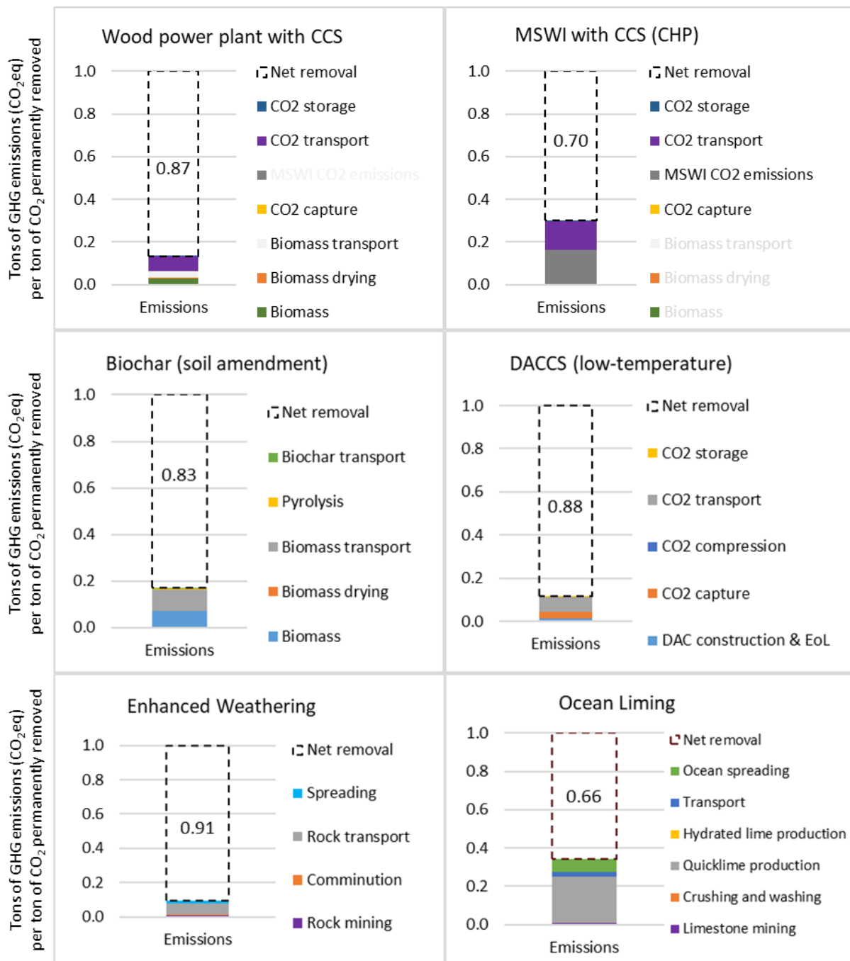
Figure 1.1: Life cycle GHG emissions of different CDR methods, evaluated with a “realistic-optimistic” parameter setting from a current Swiss perspective. MSWI: Municipal Solid Waste Incineration; DACCS: Direct Air Carbon Capture and Storage. All methods assumed to be applied in Switzerland, except Ocean Liming (Norway). Biogenic carbon content in the MSWI: 52%; all GHG emissions associated with CO 2 transport and storage are assigned to this biogenic carbon fraction, thus to the CDR service. CO 2 capture rates: 90% at the wood power plant, 85% at the MSWI plant. Spruce used as biomass feedstock for biochar production and wood combustion. Geological CO 2 storage assumed to take place in Iceland for DACCS, wood combustion and MSWI with CCS. Transport of CO 2 via pipeline over 4000km; CO 2 storage depth: 3000m. DAC operated with Swiss grid electricity and waste heat. Plant-internal heat and power supply for CO 2 capture at the wood combustion and MSWI plants. Biomass and rock transport in the range of 100km. High-temperature heat supply for quicklime production from natural gas combustion. Specific CO 2 uptake of enhanced rock weathering: 0.35 t CO 2 /t rock material. Dashed bar segments on top of each bar represent net CO 2 removal rates, i.e., the fraction of gross CO 2 permanently removed, which is not compensated by GHG emissions from the CDR product systems.
