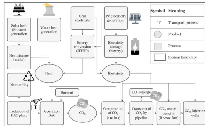
Figure 6.1: System boundaries in the LCA of DACCS according to (Terlouw, Treyer, et al. , 2021).
