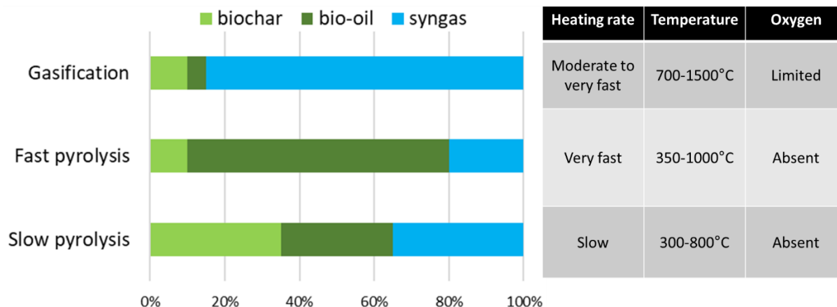
Figure 5.7: Product yields and key characteristics of biochar production processes (Hoeskuldsdottir, 2022).
