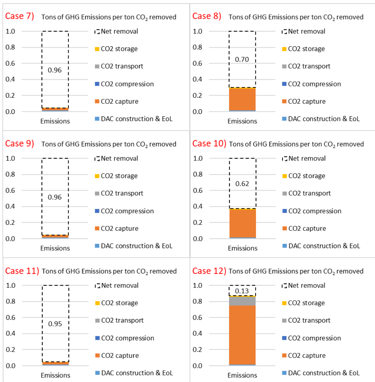
Figure 7.2: LCA results (climate impacts: tons of GHG emissions per ton of CO 2 permanently removed from the atmosphere) for different LT DACCS configurations with DAC operation in Iceland (cases 7, 8), Norway (cases 9, 10), and Greece (cases 11, 12), as generated with the LCA tool and specified above in Table 7.2. Location of CO 2 storage: Cases 7, 8, 12: Iceland; cases 9, 10: Norway; case 11: Greece. Numbers in the dashed bar segments on top of the emissions indicate net CO 2 removal rates. Cases 8, 10, and 12 use natural gas as heat source for DAC operation.
