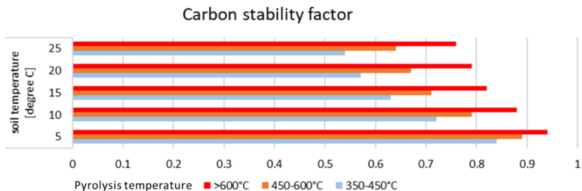
Figure 5.8: Carbon stability factor of biochar-to-soil application as a function of pyrolysis and soil temperatures (Hoeskuldsdottir, 2022) based on (Woolf et al. , 2021).
