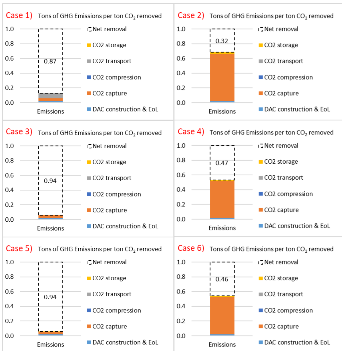
Figure 7.3: LCA results (climate impacts: tons of GHG emissions per ton of CO 2 permanently removed from the atmosphere) for different HT DACCS configurations with DAC operation in Switzerland (cases 1, 2), Norway (cases 3, 4), and Iceland (cases 5, 6), as generated with the LCA tool and specified above in Table 7.3. Location of CO 2 storage: Cases 1, 5, 6: Iceland; cases 3, 4: Norway; case 2: Switzerland. Numbers in the dashed bar segments above the emissions indicate net CO 2 removal rates. Cases 2, 4, and 6 use natural gas as high-temperature heat source for DAC operation.
