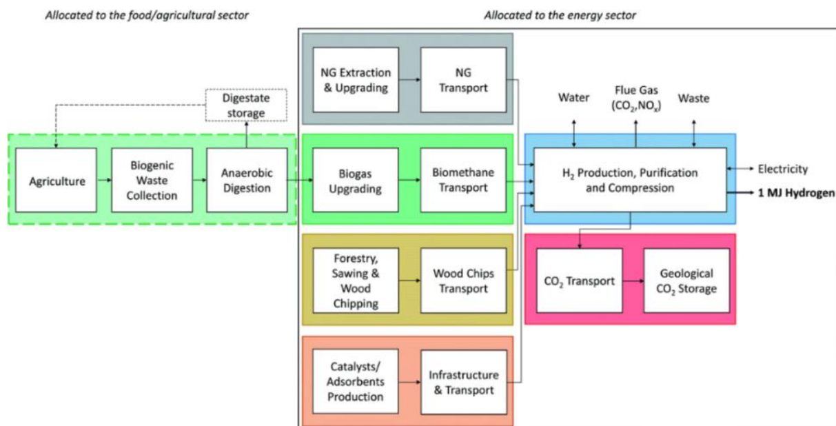
Figure 6.6: System boundaries in the LCA of hydrogen production via wood gasification and biomethane reforming with (and without) CCS (Antonini et al. , 2020, 2021).
