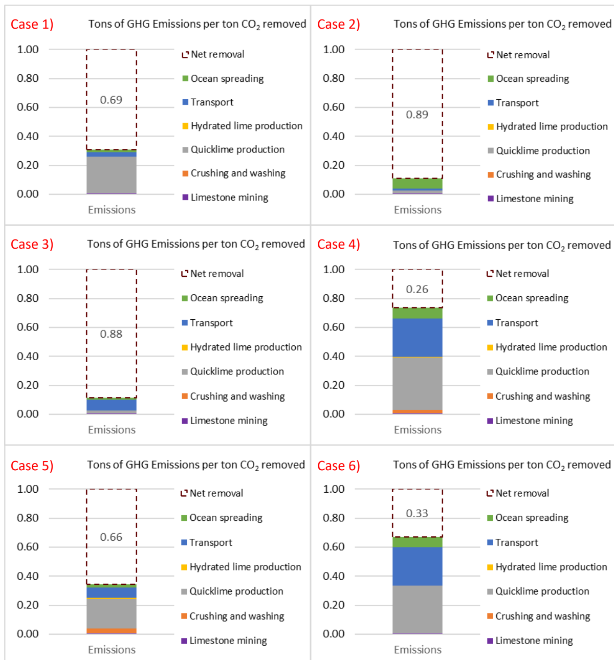
Figure 7.9: LCA results (climate impacts: tons of GHG emissions per ton of CO 2 permanently removed from the atmosphere) for different OL configurations, as generated with the LCA tool and specified in Table 7.11. Numbers in the dashed bar segments on top of the emissions indicate net CO 2 removal rates. Application in Iceland (cases 1, 2), Norway (cases 3, 4), and Greece (cases 5, 6).
