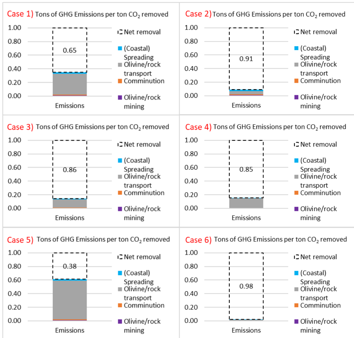
Figure 7.8: LCA results (climate impacts: tons of GHG emissions per ton of CO 2 permanently removed from the atmosphere) for different (C)EW configurations, as generated with the LCA tool and specified in Table 5.7. Numbers in the dashed bar segments on top of the emissions indicate net CO 2 removal rates. Application in Switzerland (cases 1-3), Greece (cases 4, 5), and Iceland (case 6).
