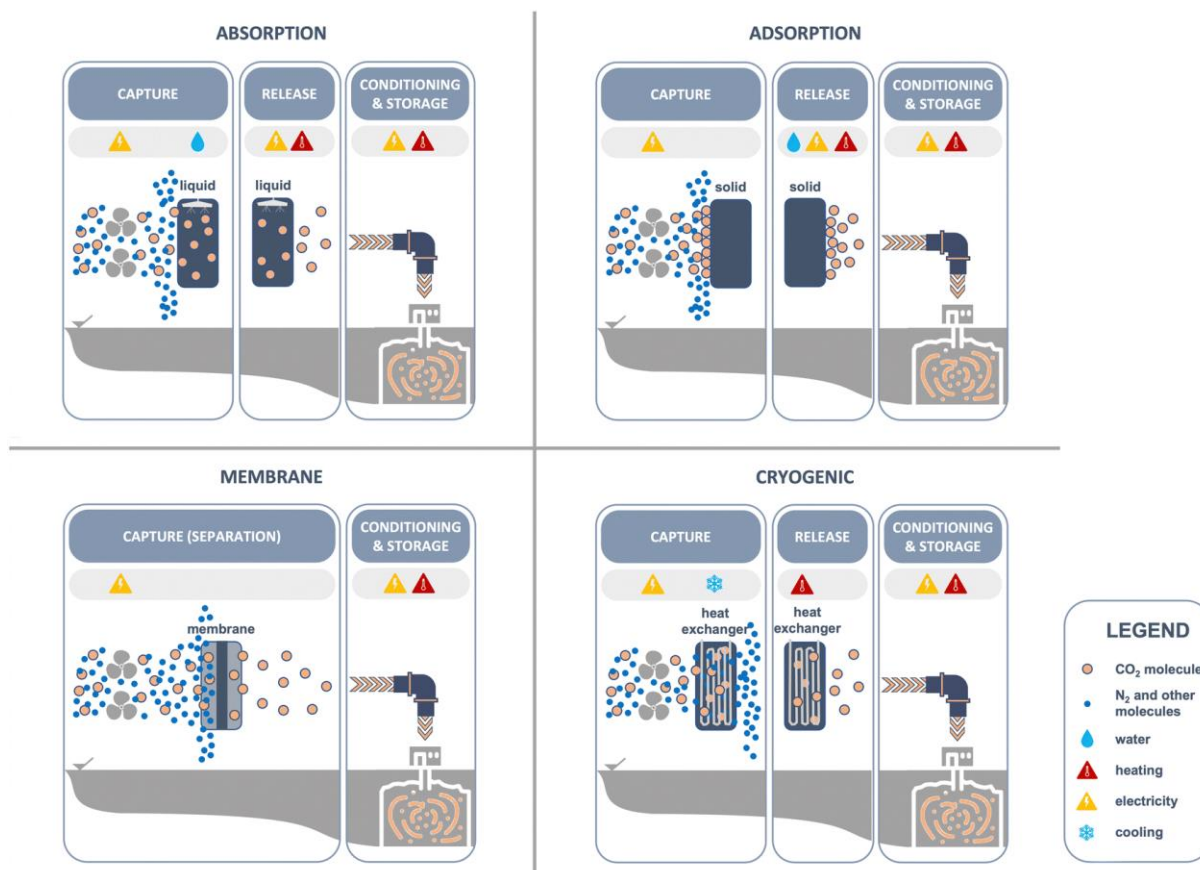
Figure 5.6: The four primary separation mechanisms in DAC processes. (i) ‘Absorption’, which works by binding the CO 2 within a liquid; (ii) ‘Adsorption’, which works by binding the CO 2 to the surface of a solid; (iii) ‘Membrane’ that separates via different diffusion abilities; and (iv) ‘Cryogenic’ process that de-sublimates (phase change from gas directly to solid without an intermediate liquid phase) CO 2 based on the higher freezing point compared to other atmospheric gases (Küng et al. , 2023).
