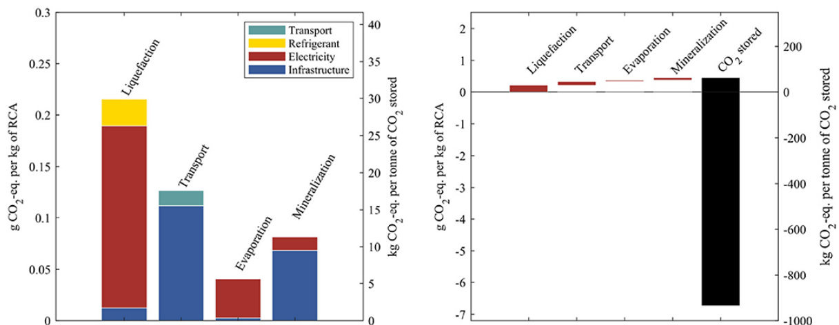
Figure 6.9: Life-cycle GHG emissions of the sub-processes of the negative emission value chain visualized along four main process categories (left) and cumulative GHG emission of the value chain, including the CO 2 removal (equal to negative emissions) of the mineralization plant (Tiefenthaler et al. , 2021).
