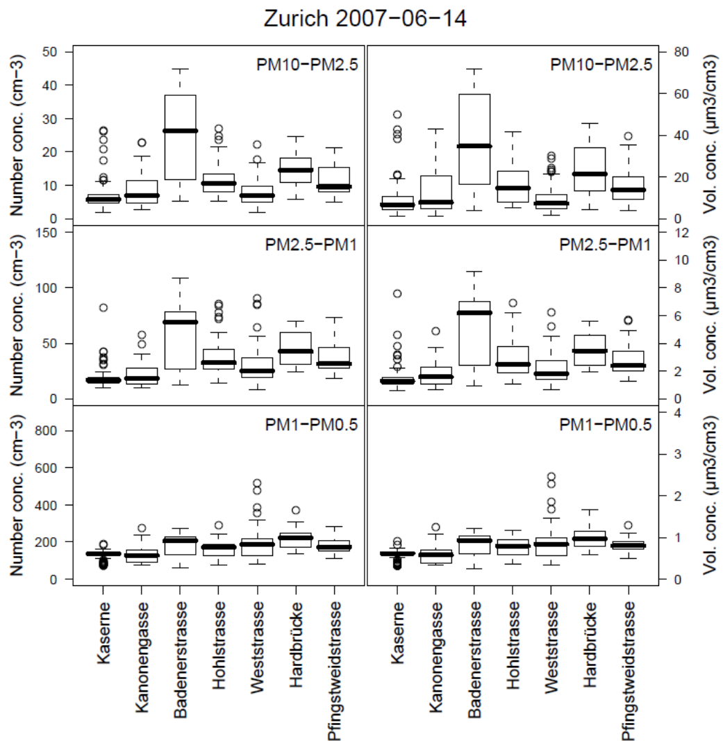
Fig. 5.5.10: Boxplot of APS particle number (left) and volume (right) concentrations for individual road sections along the test run route. The average spectra in Figure 5.5.11 exhibit a large amount of particles >10 μm (not shown).
