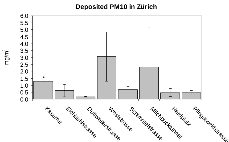
Fig. 5.3.2: Deposited total PM10 mass per \text{m}^2 for each sampling site. The black lines indicate the error bars. The sites are ordered according to increasing traffic density. Eichbühlstrasse and Kaserne are considered as background sites. See text for an explanation of the error bars. The value for Kaserne (marked with *) is based on a single filter analysis and is biased by experimental difficulties.
