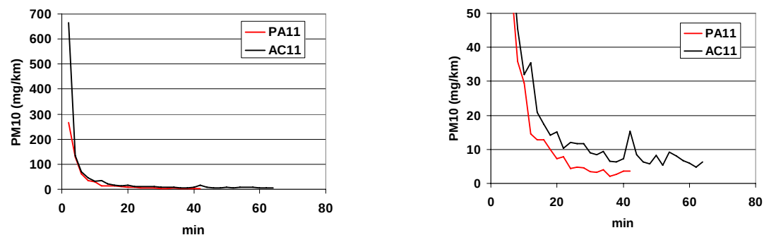
Fig. 5.2.6: Emission factors as a function of time during a MMLS (simulating LDV) abrasion experiment comparing the resuspension of fine dust from an asphalt concrete pavement (AC) and a porous asphalt pavement (PA). Left: Full scale graph. Right: Detailed view with enhanced y-axis.
