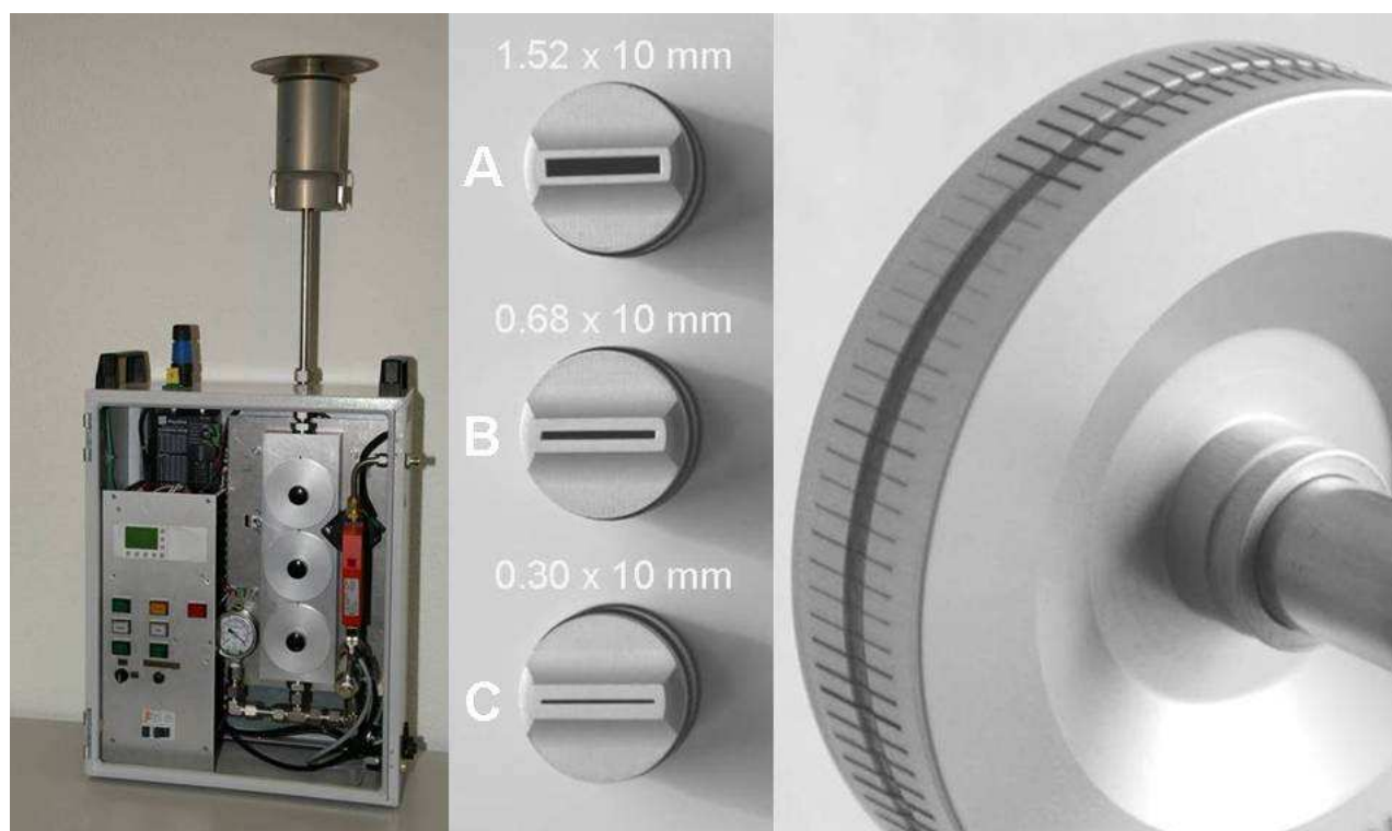
Fig. 3.3: Rotatings drum impactor (RDI) with PM10 inlet (left picture), Size-segregating nozzles of the RDI (middle), RDI sampling wheel with a sample of urban submicrometer particles (right picture). Each dark bar represents one hour of collected ambient aerosol with a total aerosol mass of approx. 10 \mu\text{g} .
