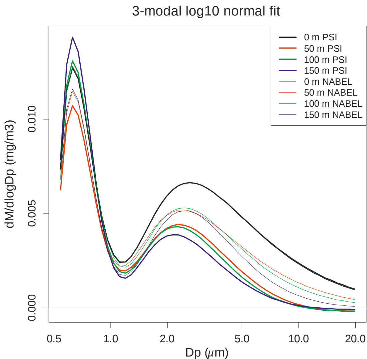
Fig. 5.4.5: APS particle mass distributions for all measured distance classes (assuming unit density). Bold lines: PSI APS data; thin lines: NABEL APS data. The NABEL APS was fixed in its location all the time, while the PSI APS was dislocated from one position to the next. Corresponding colors show the same time interval, e.g. '100 m PSI' corresponds to '100 m NABEL'. Different colors were selected for the respective distance classes, and the two instruments were distinguished with different line widths.
