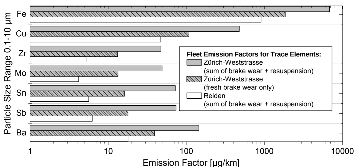
Fig. 5.1.11: Sum fleet emission factors (particle size range 0.1 - 10 µm) for Zürich-Weststrasse (10% HDV) and Reiden (15% HDV), for trace elements associated to brake wear. The values for Zürich-Weststrasse were calculated from experimental data from February and March 2007 (9 days, dry time periods only), while the values for Reiden refer to October 2007 (4 days, dry time periods only).
