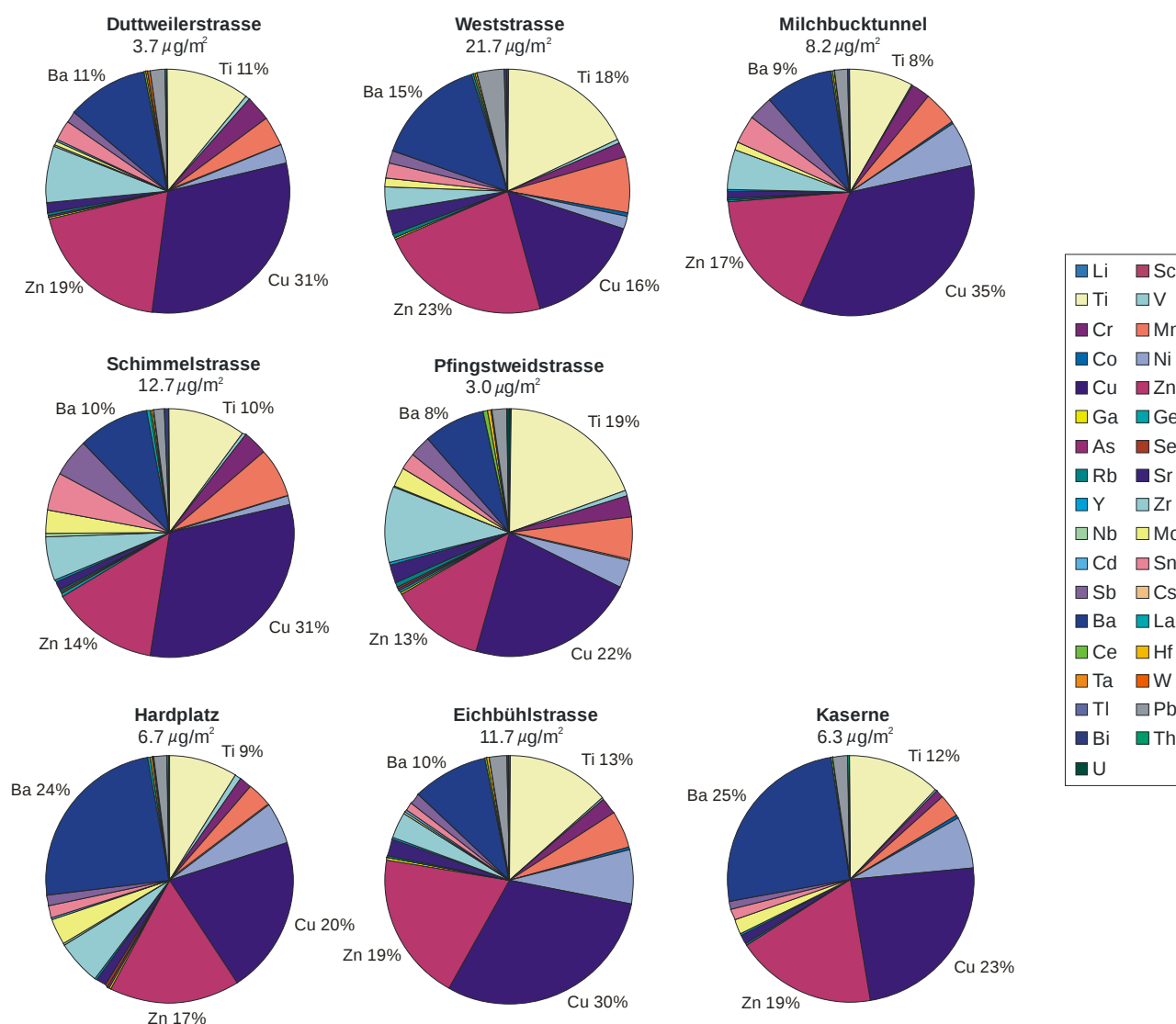
Fig. 5.3.5: Relative abundances of trace elements present in deposited PM10 in Zurich. The numbers under the site names indicate the total mass per m² of the considered trace elements.
