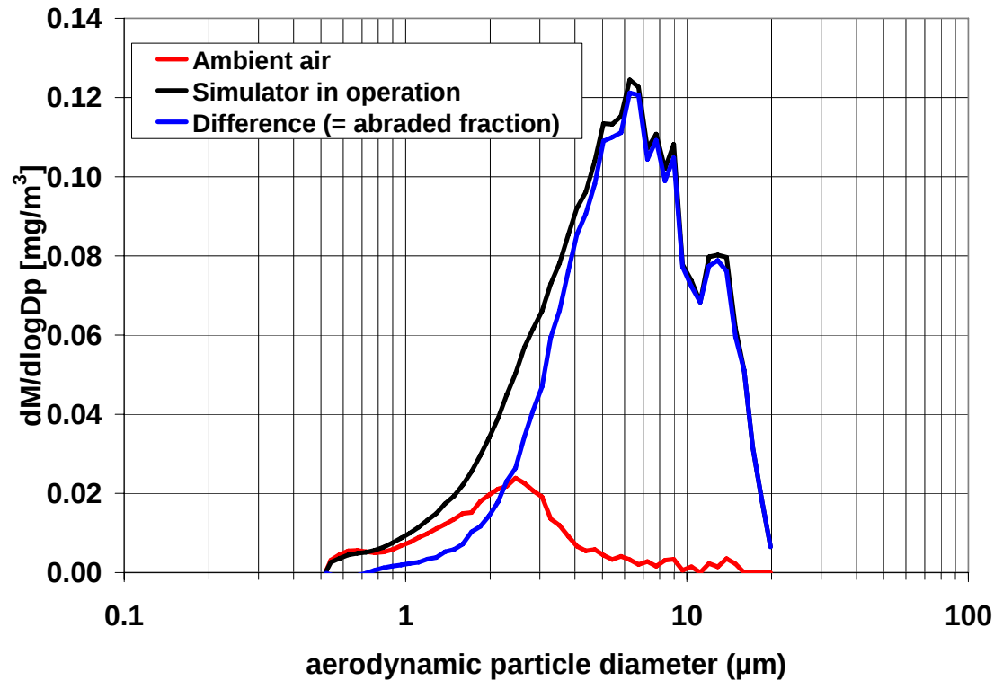
Fig. 5.2.1: Typical particle size distribution obtained from an experiment with the mobile load simulator, during a measurement period with dominating abrasion (negligible resuspension). The size distribution of the abrasion particles is clearly shifted towards the coarse side compared to the ambient size distribution.
