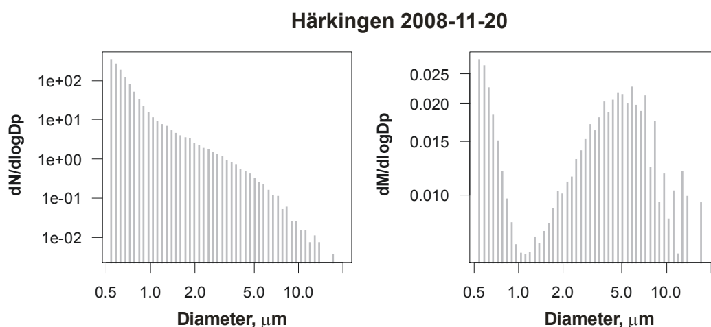
Fig. 3.15: Example size spectrum measured with the PSI Aerodynamic Particle Sizer spectrometer (APS). Left: Particle number concentration dN/d\log D_p in counts. Right: Mass concentration dM/d\log D_p in \text{mg m}^{-3} .
