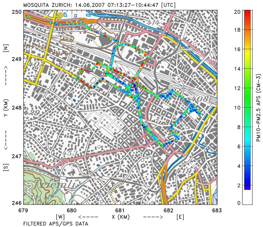
Fig. 5.5.9: Mosquita test run on 14 June 2007 0713-1045 UTC, showing number concentrations for particles with diameters 2.5 – 10 \mu\text{m} .
