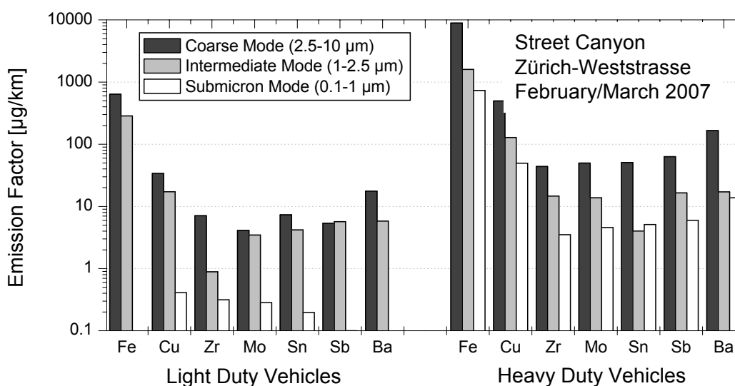
Fig. 1.7: Light duty vehicle (LDV) and heavy duty vehicle (HDV) emission factors (EF) for Zürich-Weststrasse (street canyon). The calculation was performed using 209 hourly values ( \sim 9 days, \Delta\text{NO}_x > 20 \mu\text{g m}^{-3} , dry time periods only). For Zn no emission factors were calculated because the significant presence of other sources for this element did not allow for the determination of the contribution of local road traffic within the street canyon.
