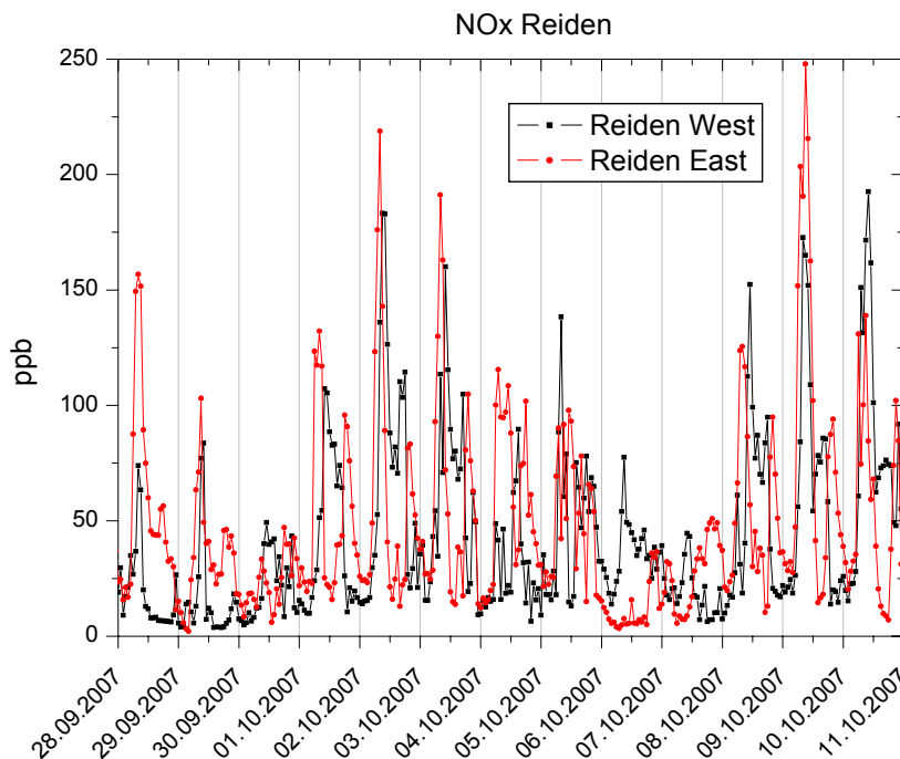
Fig. 5.6.23: Extract of time series for \text{NO}_x at both stations in Reiden.
