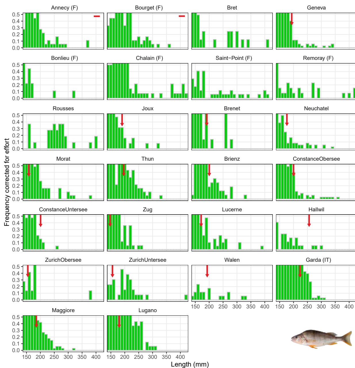
Figure 9: Length frequency distribution of large perch among lakes. Data from benthic CEN nets to 20 meters deep. The number of fish is adjusted for the corresponding gillnetting effort in the lake. Vertical axis is truncated at 0.5 fish per 100 m 2 of net to focus on the occurrence of the larger fish. Arrows indicate the approximate length of fish at which permitted nets for commercial fisheries become efficient. There was no commercial fishing in lakes Bret, Bonlieu, Chalain, Saint-Point, Remoray and Rousses at the time of Projet Lac sampling. No minimum size limit for perch in Annecy and Bourget. Lakes Biel and Sarnen are excluded as the different mesh sizes used in the Projet Lac sampling of these lakes influences the fish length frequency distribution, meaning that it is not possible to directly compare them to other lakes.
