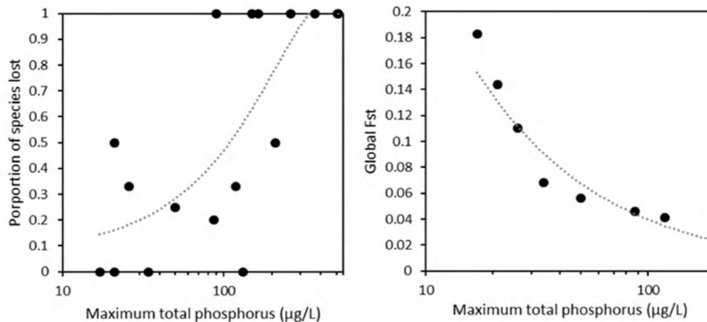
Figure 24: Relationship of the maximum total phosphorus concentration experienced by each lake versus the proportion of Coregonus species lost in each lake (left) and the genetic differentiation (global Fst) among the post-eutrophication Coregonus species within those lakes that retain native Coregonus species (right). Modified from [42].
