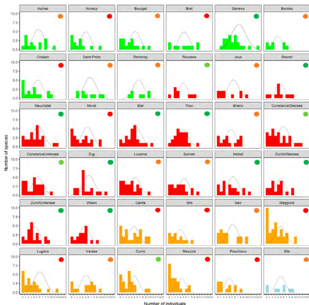
Figure 6: Species-abundance distributions (SADs) for each of 35 perialpine lakes and 1 lowland lake. These SADs result from combining partial SADs obtained by sampling with the CEN netting protocol, the VERT netting protocol and the electrofishing protocol (for all partial SADs see Appendix B Figure 69). Abundances are log2-transformed. Normal distributions are indicated by a thin line in each plot. The qualitative fit to the expected distribution is indicated by coloured circles: dark green = good fit, light green = modest fit, orange = poor fit, red = very poor fit. Colour of bars indicates drainage systems: green = Rhône, red = Rhine, orange = Po, blue = Danube. Note the systematic difference between Rhine lakes (9 good, 3 modest, 4 poor, 1 very poor) and Po lakes (0 good, 1 modest, 2 poor, 6 very poor). This difference cannot be due to differences in sampling effort because Maggiore and Lugano were among the best sampled lakes, but both have very poor fits to the expected distributions. Lake Aulnes is a lowland lake in the southern Rhône drainage that we sampled but did not otherwise consider in this report.
