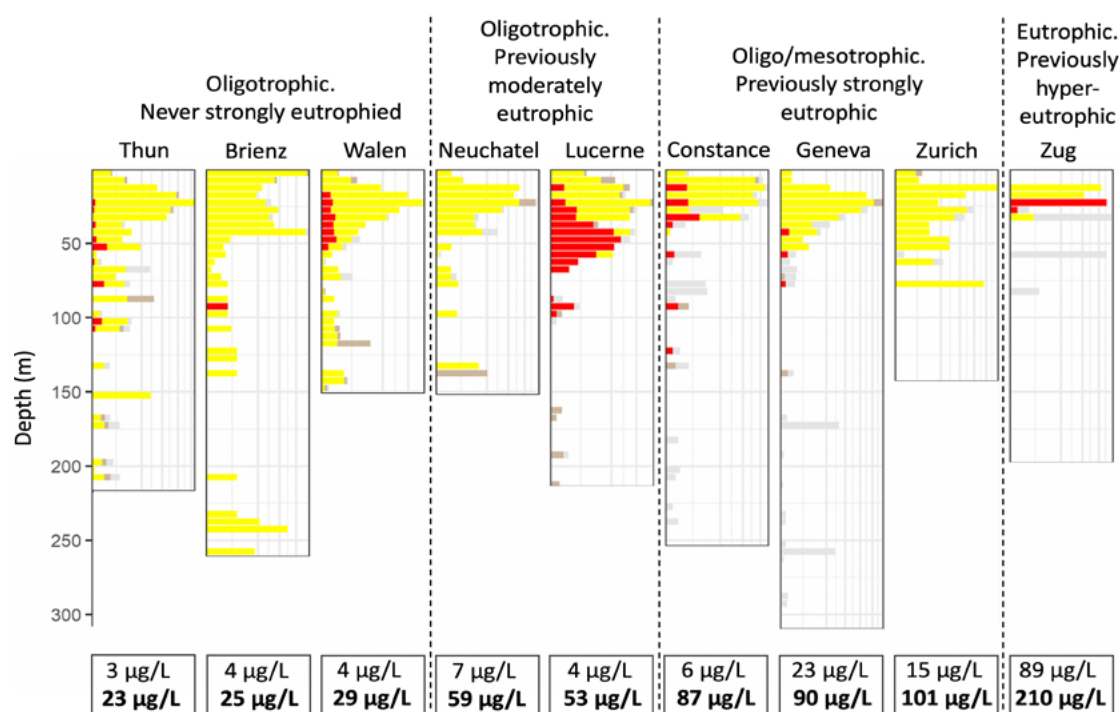
Figure 26: Depth distribution of catch per unit effort (CPUE; horizontal axis) for native fish species living in the deeper zones of the deep, northern perialpine lakes: Coregonus spp (yellow), Salvelinus spp (red), Cottus spp (grey/brown) and Lota lota (light grey). CPUE is the average of catches in deep-set vertical nets and benthic CEN nets. CPUE is square-root transformed to increase the visibility of the smaller values in the profundal zone. Note that the scale of the horizontal axis (CPUE) differs among the lakes. Whereas Lota lota has pelagic eggs and larvae and does hence not have to recruit locally, all other species recruit locally. Boxes at the bottom of the figure show the total phosphorus of the lake at the time of Projet Lac sampling (upper value) and the maximum measured total phosphorus value that had been experienced by the lake in the past (lower value in bold). The panels for Constance and Zurich show the data for the deeper lake in each of the pairs (i.e. Upper Constance and Lower Zurich).
