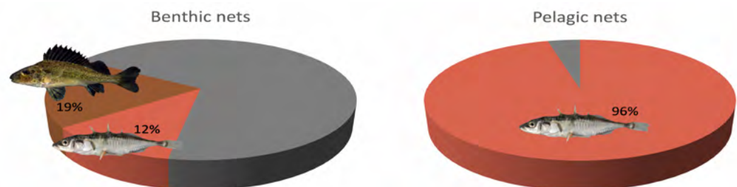
Figure 27: Contribution of two non-native fish species, Gasterosteus aculeatus (pink) and Gymnocephalus cernua (brown), to fish abundance in CEN gillnets set in the benthic (left) and pelagic (right) zones of Upper Lake Constance. The proportion of native species is represented in grey.
