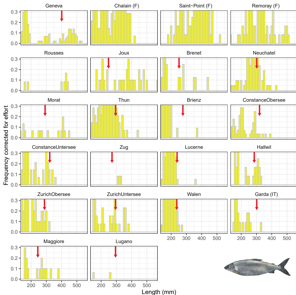
Figure 8: Length frequency distribution of Coregonus spp among lakes. Data from deep-set vertical nets (set deeper than 5 m). The number of fish is adjusted for the number of vertical net batteries deployed in the lake. Vertical axis is truncated at 0.3 fish per vertical net battery to focus on the occurrence of the larger fish. Arrows indicate the approximate length of fish at which permitted nets for commercial fisheries become efficient. There was no commercial fishing in lakes Chalain, Saint-Point, Remoray and Rousses at the time of Projet Lac sampling. Lakes Biel and Sarnen are excluded as the different mesh sizes used in the Projet Lac sampling of these lakes influences the fish length frequency distribution, meaning that it is not possible to directly compare them to the other lakes.
