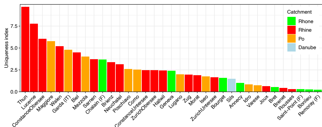
Figure 10: Uniqueness of the fish communities of all lakes and catchments. Uniqueness index for each lake was calculated as the sum of the inverse of the number of lakes where each species in the lake was recorded.
