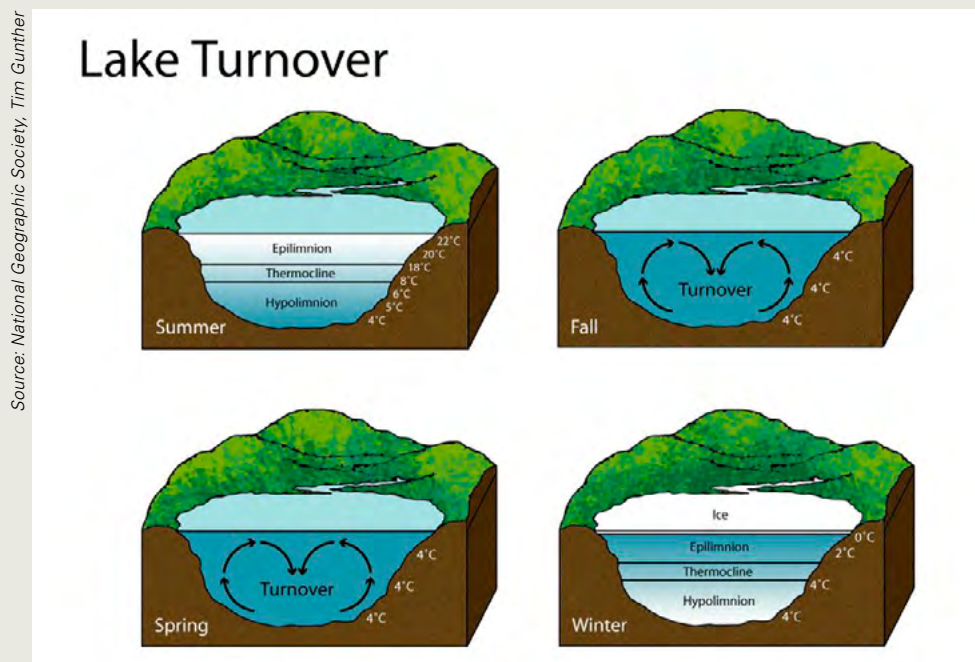
Figure 90: Representation of the seasonal cycle of stratification and mixing in a dimictic lake throughout a year.
