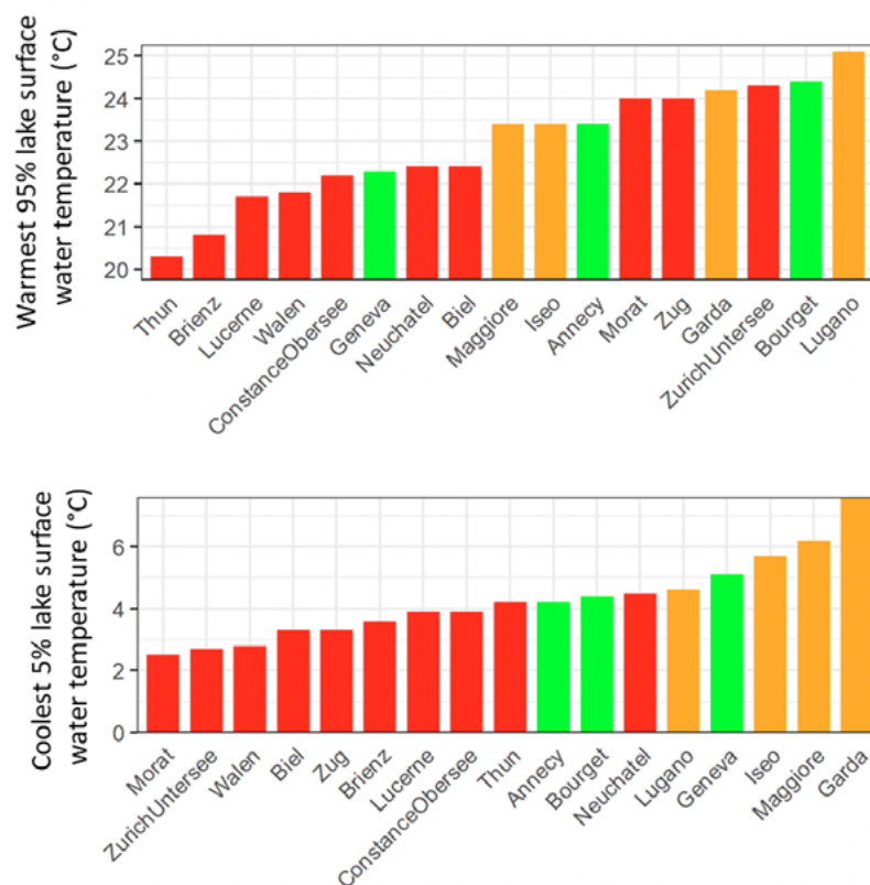
Figure 88: Water temperature in lakes of the Po river catchment (orange) were generally warmer than in lakes of the Rhine (green) and Rhine (red) catchments. The lakes on the northern edge of the Alps remain cooler in summer and the lakes in the south remain warmer in winter. Upper panel shows 95 % quartile and lower panel shows 5% quartile of monthly mean lake surface water temperatures based on remote sensing (Advanced Very High Resolution Radiometer; 1989 – 2014 [214] ). Quartiles were used rather than true minimum/maximum to avoid the effects of outliers.
