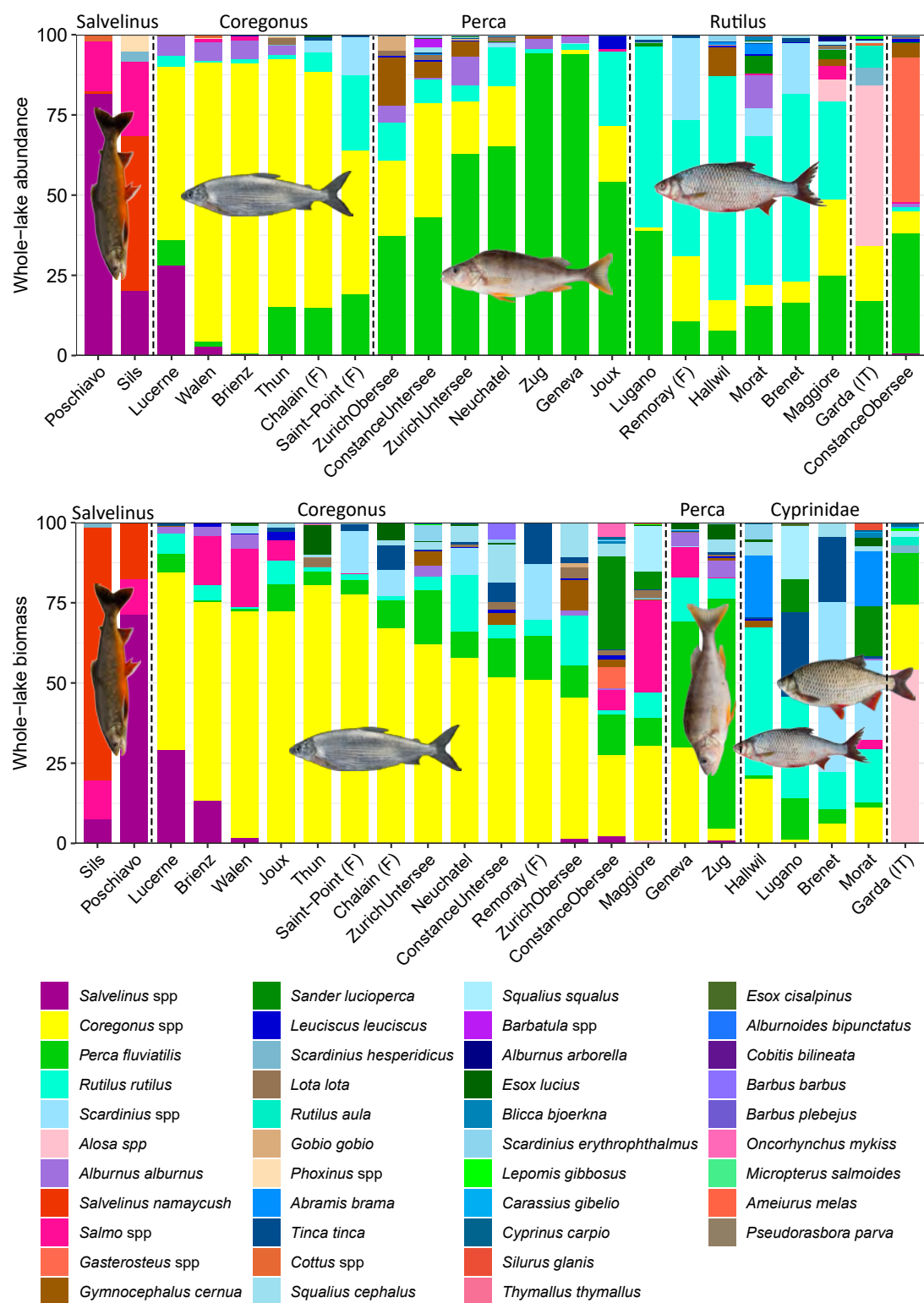
Figure 7: Whole-lake community composition based on CPUE in vertical nets. Upper panel shows volume-weighted average number of fish per 100 m² net area. Lower panel shows volume-weighted average biomass per 100 m² net area. Figure includes only lakes surveyed by the standard vertical net protocol. Lakes Sarnen and Biel were sampled with a modified protocol and are excluded here. The smallest lakes Bret and Bonlieu are also excluded. Note that sequence of lakes along the X axis differs between the panels.
