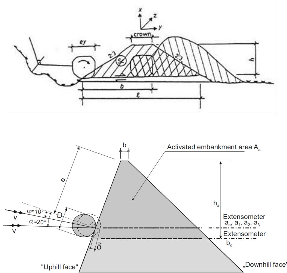
Figure 27 Model of the impact disturbed zone (IDZ) considered by Tissières (1999) (top) and by Hofmann and Mölk (2012) (bottom).
