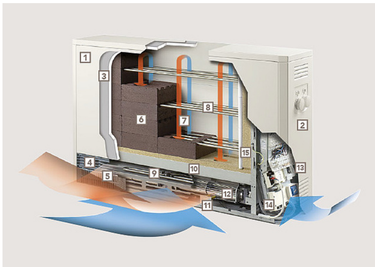
Figure 11: Schematic representation of the structure and components of an AEG night storage heater (Energie Experten, Greenhouse Media GmbH, 2016)
