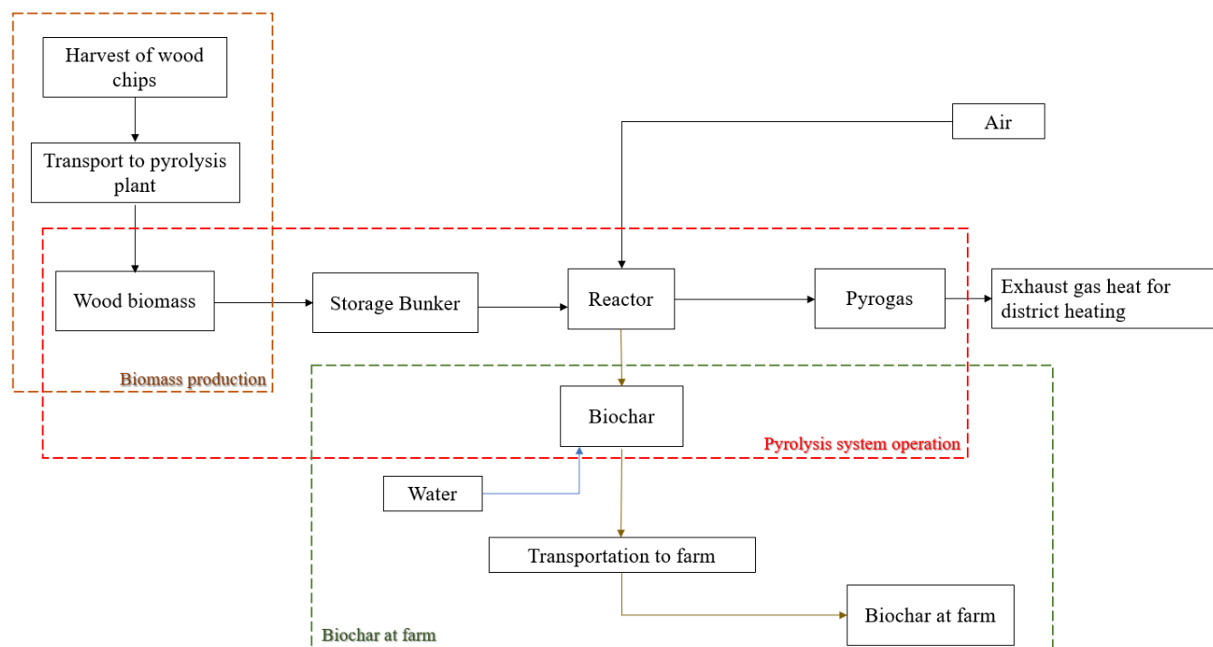
Figure 3: Overview of the core and main processes for the biochar production in the pyrolysis plant.
