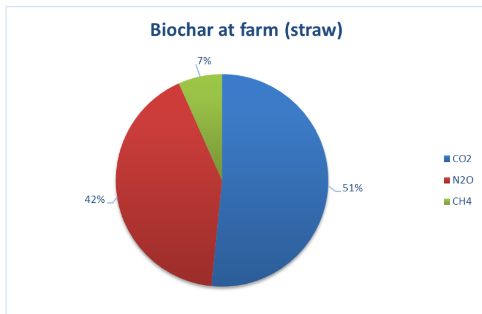
Figure A8: Contributions (%) of CO 2 , CH 4 and N 2 O to the Global Warming Potential of the LCI "Biochar at farm", biochar produced with straw (processes included: biochar(straw), tap water, transport-freight lorry).
